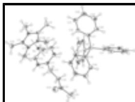
Fig. 1. The structure of the cation and anion of (I), with atom labels and 40% probability displacement ellipsoids for the non-H atoms.
